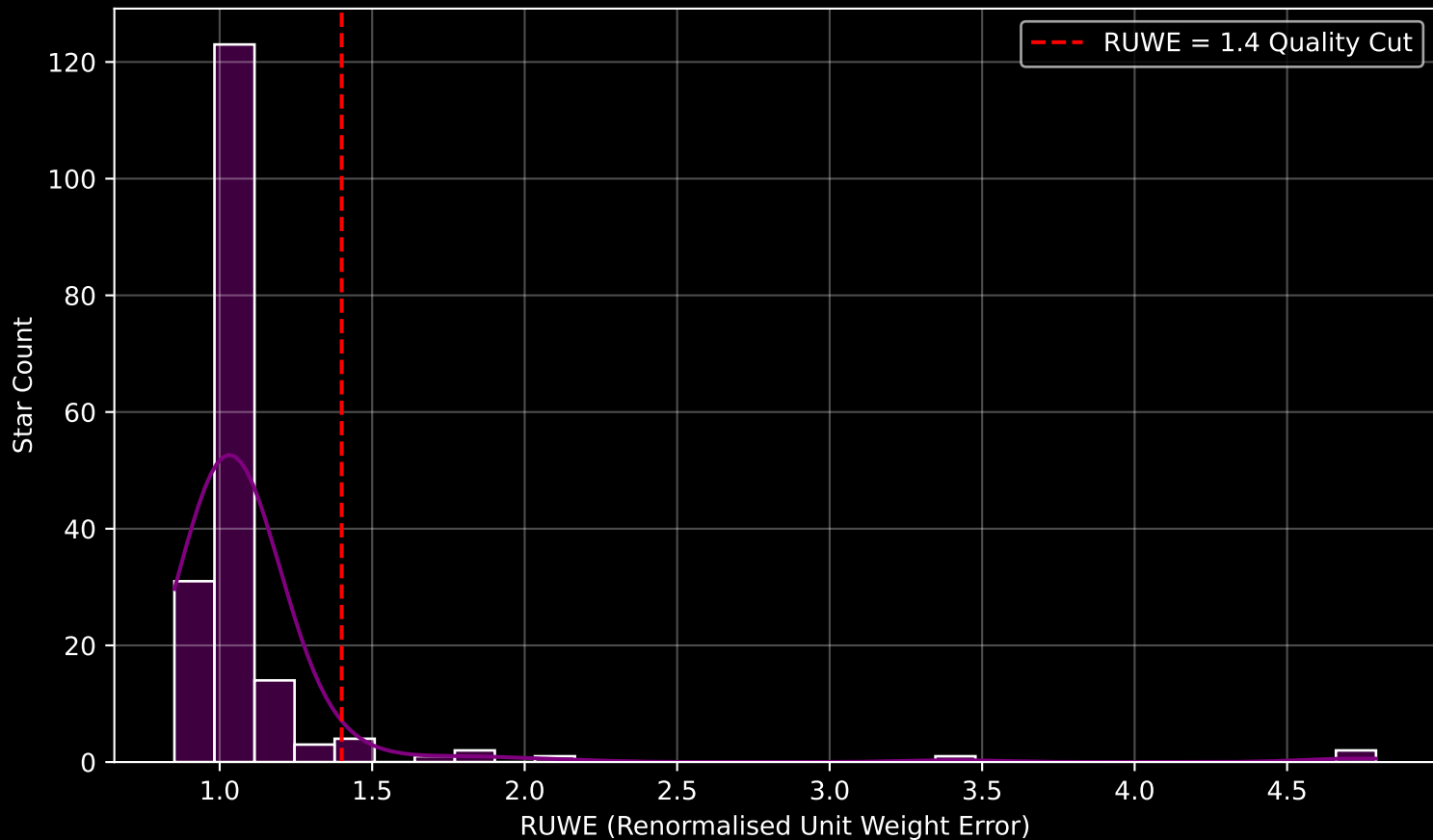
GAPOGEE DR17 Field [131+04] RUWE Distribution (n= 182)
