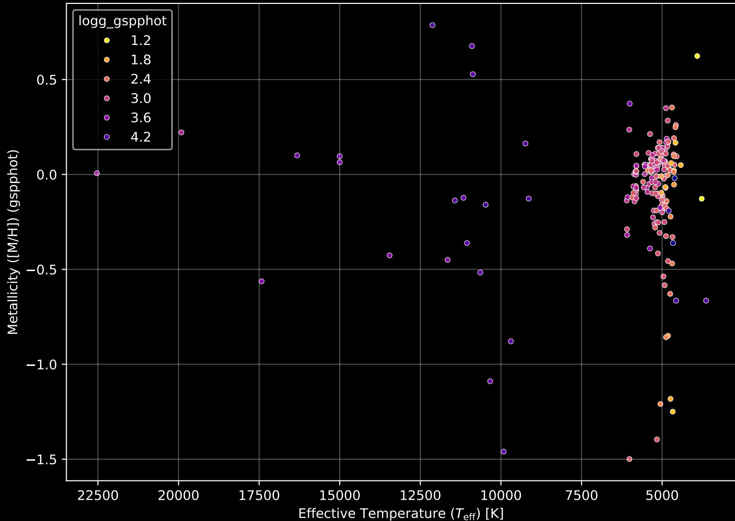
APOGEE DR17 Field: [131+04] Stellar Population Parameters (n= 185)
