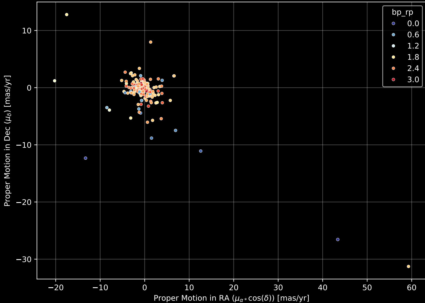
APOGEE DR17 Field: [131+04] Proper Motion Diagram (n= 185)
