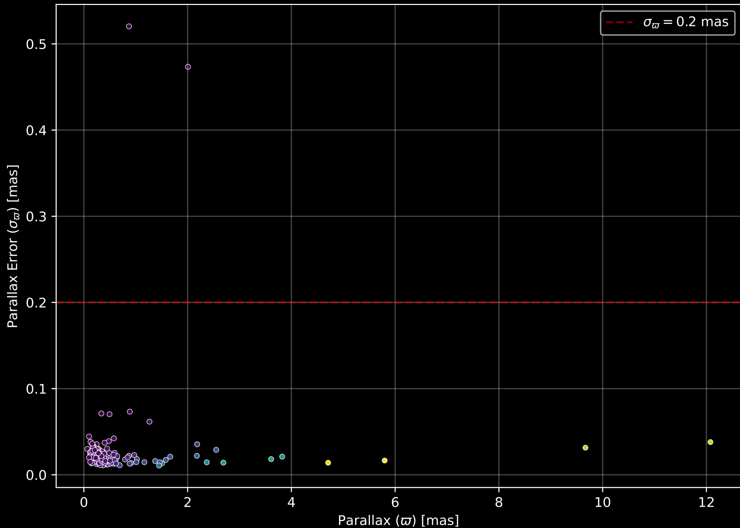
APOGEE DR17 Field: [131+04] Parallax Quality (n= 185)
