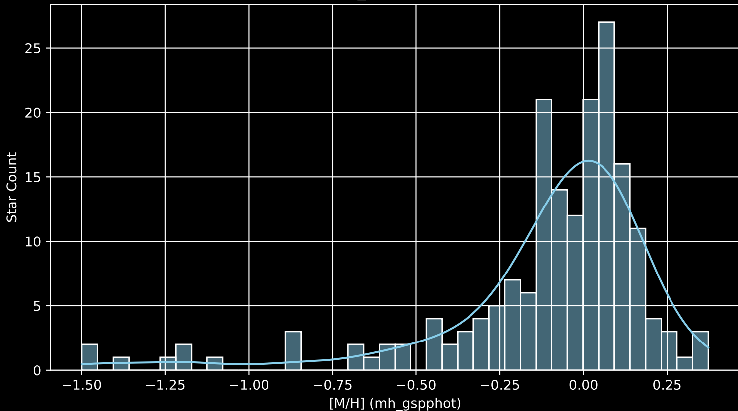
APOGEE DR17 Field: [131+04 [M/H] (mh_gspphot) (n= 181)
